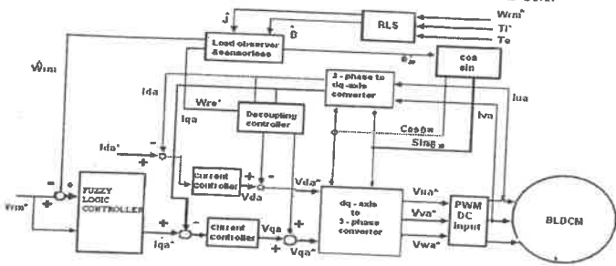
Fig. 3. Block diagram of sensorless speed control of BLDCM.
