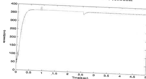
Fig. 7. Simulated speed response of system with PI controller
