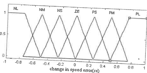
5. Plot of membership function for change in speed error
