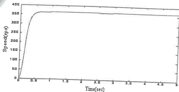
simulated speed response of system with Fuzzy controller
