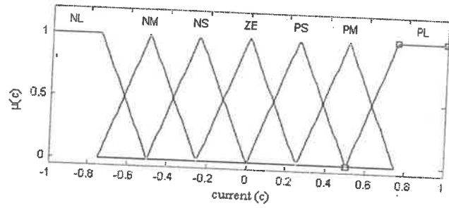
Fig. 6. Plot of membership function for current
