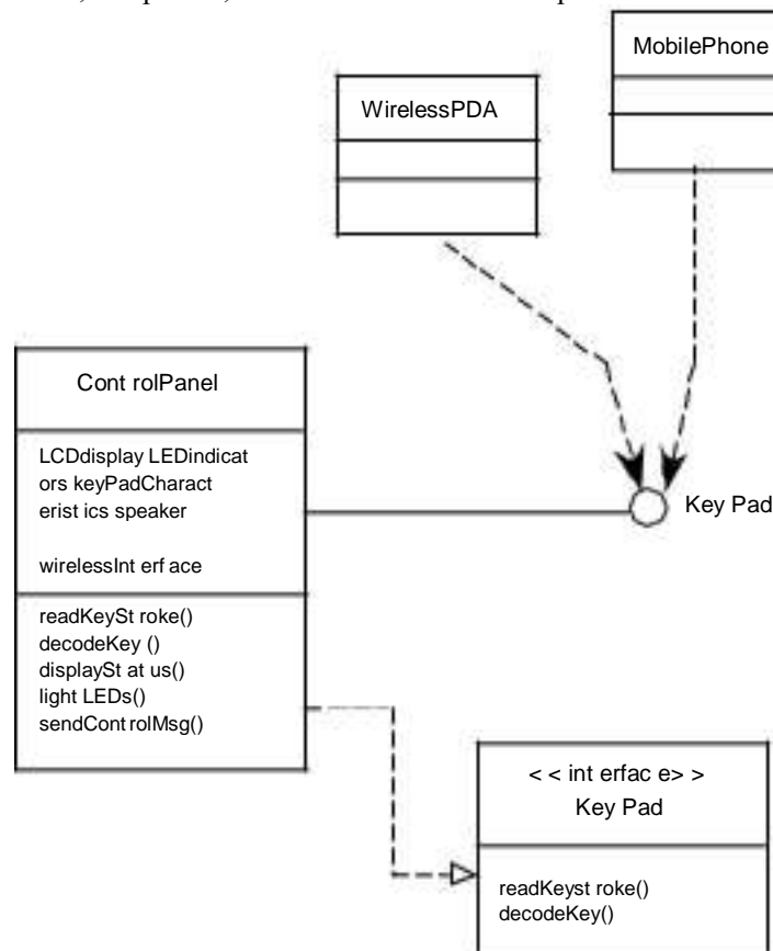
Figure 9 . 6 UML int erf ace represent at ion for Co n t r o l P a n e l
